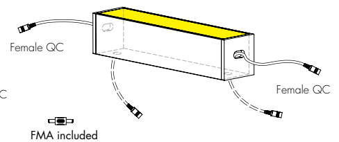
4 Dual Female Quick Connect
