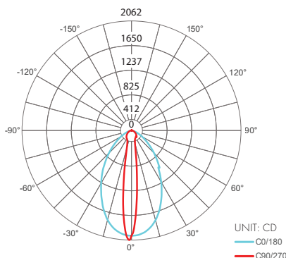
KM-48-72VHO-30K-GR Kendo M, 4ft, 3500K, 72VHO, Narrow Beam Grazer Lens
